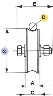
Art. 363 in acciaio zincato en acier galvanisé galvanized steel hierro cingado
